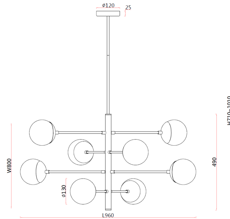
3087-8P ⊖ 960 ⊕ 800 ⓘ 710/1010 ⓘ 8 x G9 x 25W metal, glass
